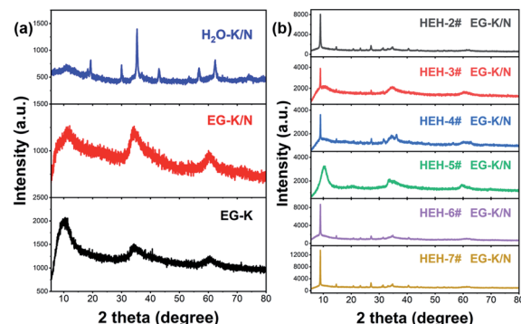
Fig. 1 (a) XRD patterns of the HEH-1# as-synthesized products under H 2 O-K/N, EG-K/N, and EG-K synthesis conditions. (b) XRD patterns of HEH-2#–7# as-synthesized products under EG-K/N conditions. All samples were synthesized by solvothermal treatment at 200 °C for 2 h.
