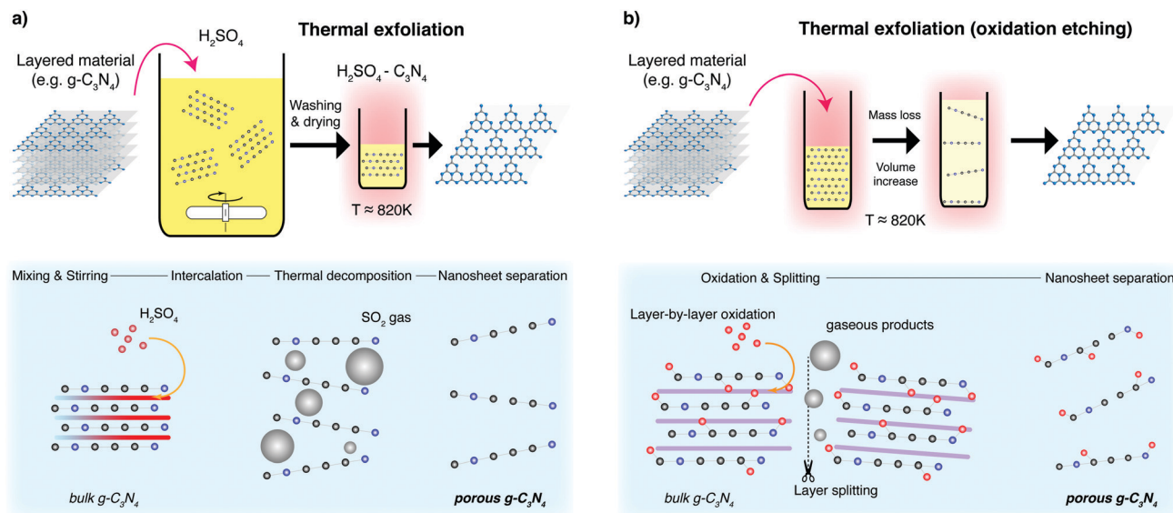
Fig. 14 Synthesis of nanosheets using thermal exfoliation can be achieved through a variation of thermal treatment approaches. (a) Intercalation of H 2 SO 4 between layers leads to the formation of gas bubbles during the heating and thermal decomposition step, leading to the separation of nanosheets. (b) Thermal decomposition in air leads to layer-by-layer oxidation and layer splitting processes with gaseous products released. Fragmentation of nanosheets, together with the formation of pores and defects, also occur using these approaches.
