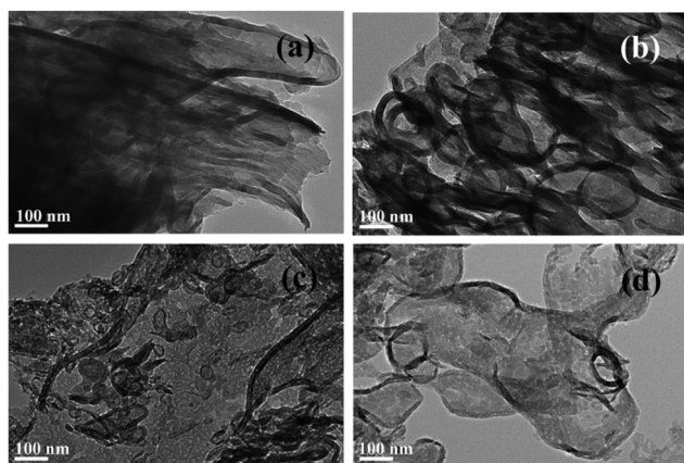
Fig. 15 TEM images of bulk g-C 3 N 4 (a), alongside porous g-C 3 N 4 exfoliated at 450 °C (b), 500 °C (c), 550 °C (d). The heat decomposes certain areas of the nanosheets, leaving the resultant sheets ranging from slightly exfoliated and porous to fully exfoliated and with large holes. Reproduced with permission from ref. 188. Copyright 2015 Elsevier B.V.
