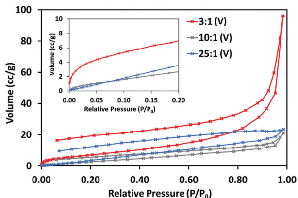
Fig. 6 \text{N}_2 adsorption-desorption isotherms for 3 : 1 (V), 10 : 1 (V) and 25 : 1 (V), at 77 K, with section of low pressure adsorption up to 0.20 P/P_0 (inset).
