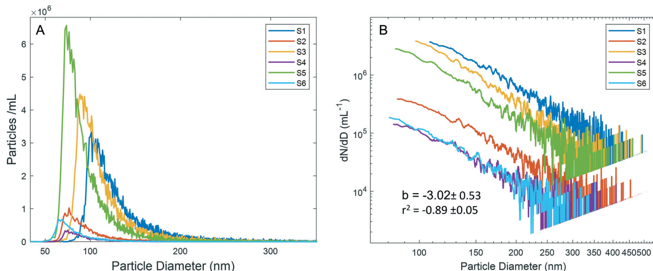
Fig. 2 A) Particle size distributions for ^{27}\text{Al} obtained by spICP-QMS. B) Reprocessed PSD data, with data normalized to number per nm ( \text{dN/dD} ) versus diameter and plotted in log space. The slope ( b ) and r^2 are an average of all samples; \pm 1 SD.
