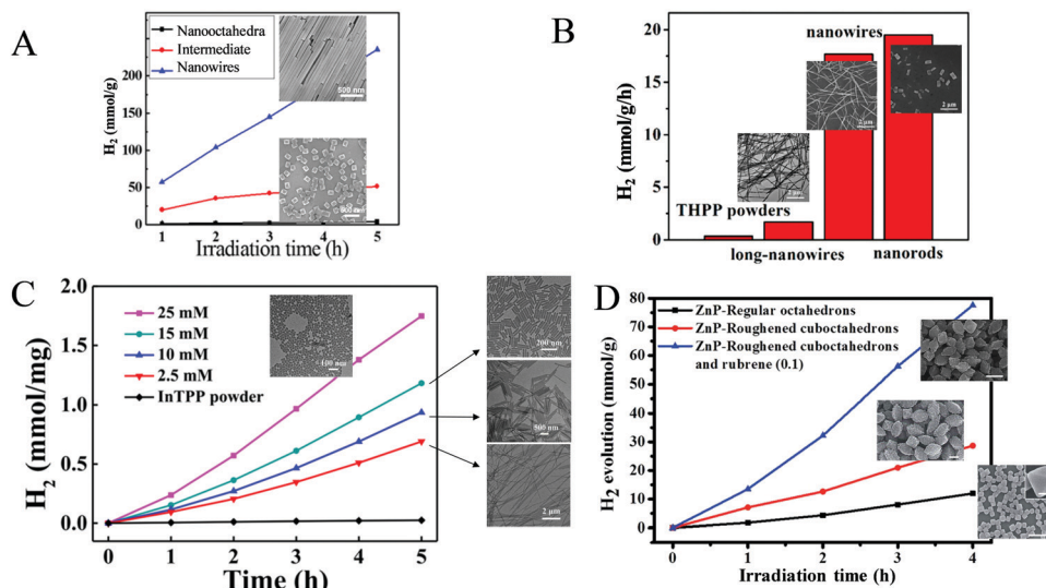
Fig. 12 (A) \text{H}_2 evolution plots of ZnTPyP self-assemblies. Reproduced from ref. 64, with permission from American Chemical Society, Copyright 2016. (B) Amount of \text{H}_2 evolution of THPP nanowires. Reproduced from ref. 66, with permission from American Chemical Society, Copyright 2018. (C) \text{H}_2 production experiments of different InTPP nanocrystals. Reproduced from ref. 67, with permission from American Chemical Society, Copyright 2019. (D) \text{H}_2 evolution plots of ZnTPP self-assemblies. Reproduced from ref. 68, with permission from Royal Society of Chemistry, Copyright 2017.
