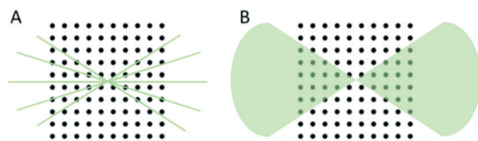
Fig. 1 Schematic illustration of (A) stepwise and (B) continuous rotation methods for 3D ED data collection. Stepwise methods sample the reciprocal space discretely with point intensities of the reflections are recorded. Continuous rotation methods sample the reciprocal space continuously and take an integral of the intensities over the exposure time.
