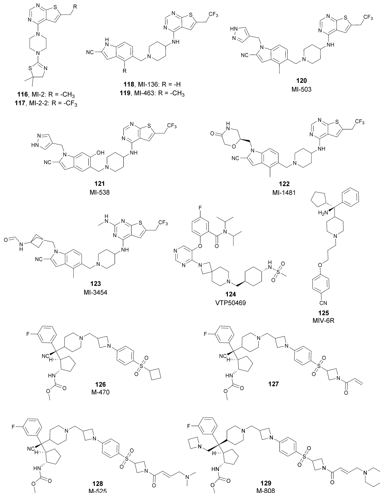
Fig. 34 MLL–menin interaction disruptors.
