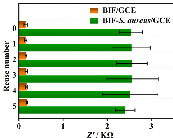
Fig. 7 Reusability of the BIF-based sensing interface. The impedance of BIF/GCE before and after the recognition of S. aureus ( 10^5 CFU \text{mL}^{-1} ) with different reuse numbers.
