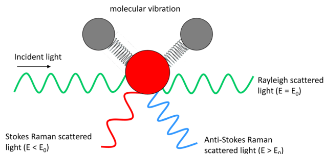
Fig. 1 Raman scattering schematic.
