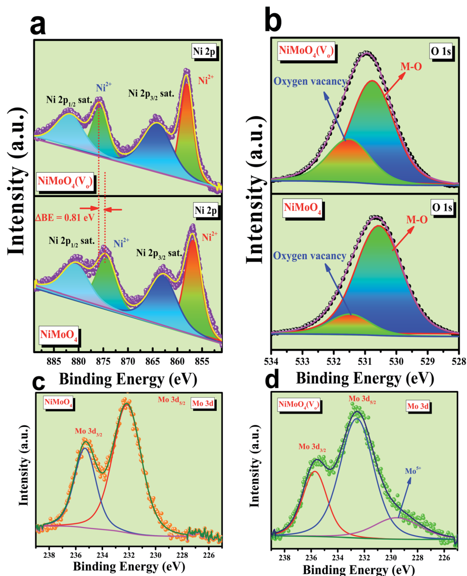
Fig. 5 (a) Combined high-resolution XPS spectra of Ni 2p orbitals for \text{NiMoO}_4 and \text{NiMoO}_4(\text{V}_\text{o}) , (b) deconvoluted XPS spectrum of O 1s orbitals, (c) XPS spectra of Mo 3d orbital of \text{NiMoO}_4 and, (d) XPS spectra of Mo 3d orbital of \text{NiMoO}_4(\text{V}_\text{o}) .
