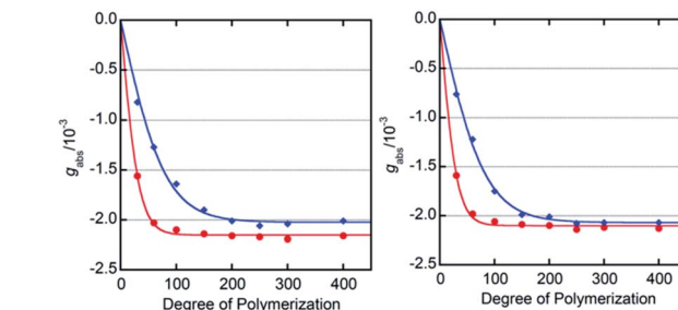
Fig. 3 CD intensities ( g_{\text{abs}} at 367–371 nm at 293 K) of PQX(n) ( \text{ca. } 7 \times 10^{-4} M based on monomer units, n = 30, 60, 100, 150, 200, 250, 300 , and 400) in THF ( \blacklozenge ) and MTBE ( \bullet ) in the presence of TFAc-L-Pro-OMe (left) and Ac-L-Pro-OMe (right) (10 mol%).
