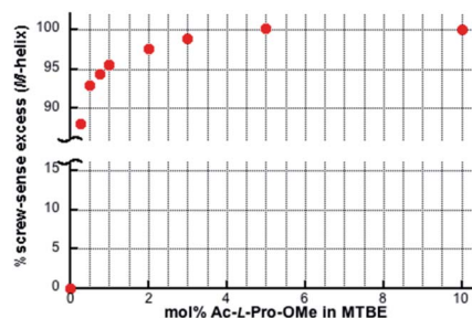
Fig. 4 Screw-sense excesses of PQX(1000) ( \text{ca. } 7 \times 10^{-4} M based on monomer units) in MTBE in the presence of Ac-L-Pro-OMe with varied concentrations.
