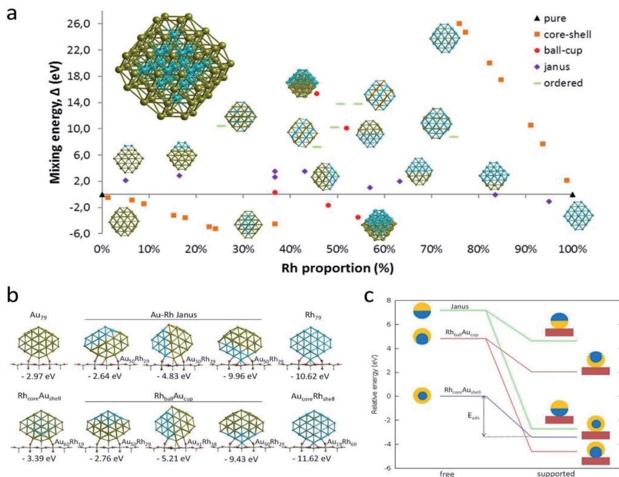
Fig. 9 (a) Mixing energy versus atomic composition for 79-atom Au–Rh nanoalloy TO clusters and monometallic counterparts. The most stable cluster ( \text{Rh}_{19}\text{@Au}_{60} ) is enlarged in inset. (b) Structure and corresponding adsorption energy for clusters of selected compositions adsorbed on \text{TiO}_2(110) . Blue, yellow, cyan, and red spheres represent Rh, Au, Ti, and O atoms, respectively. Only one layer of the \text{TiO}_2 slab is shown for simplicity. (c) Schematic view of the energetics of free and supported \text{Au}_{50}\text{Rh}_{29} clusters. This figure is reproduced from ref. 122 with permission from Scientific Reports , copyright 2016.
