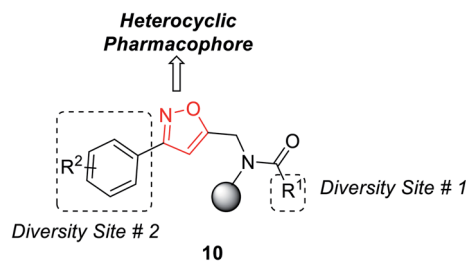
Fig. 3 Diversity points of substituted isoxazoles.
