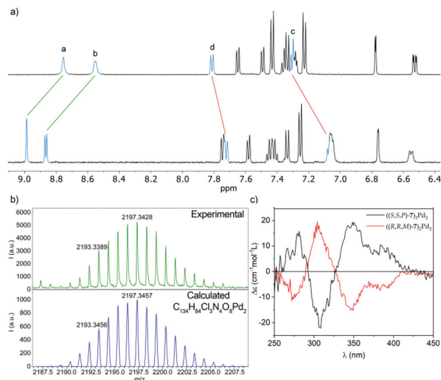
Fig. 9 (a) Partial ^1\text{H} NMR (500 MHz, \text{CD}_2\text{Cl}_2 ) spectra of ligand ((S,S,P)-7)_2 (top) and metallocupramolecular complex ((S,S,P)-7)_2\text{Pd}_2 (bottom). The lettering corresponds to that shown in Fig. 1; (b) observed (top) and calculated (bottom) HRMS (MALDI ^+ ) isotopic pattern for the [\text{M} - \text{Cl}]^+ ion of metallacycle ((S,S,P)-7)_2\text{Pd}_2 ; (c) ECD spectra of complex ((S,S,P)-7)_2\text{Pd}_2 (black line) and its enantiomer ((R,R,M)-7)_2\text{Pd}_2 (red line).
