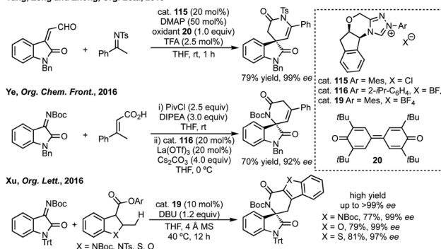
Scheme 73 NHC catalysed cycloadditions to spiro- \delta -lactams.
