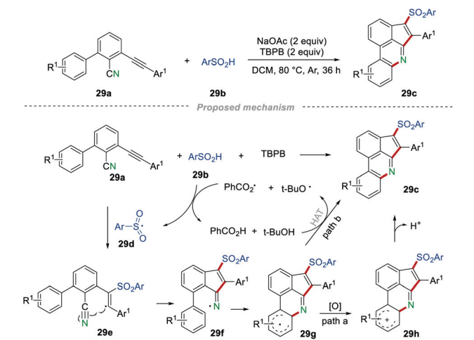
Scheme 29 The construction of 3-sulfonated cyclopenta[gh]phenanthridines.
