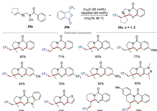
Scheme 25 The preparation of trifluoromethylated quinazolinones.
