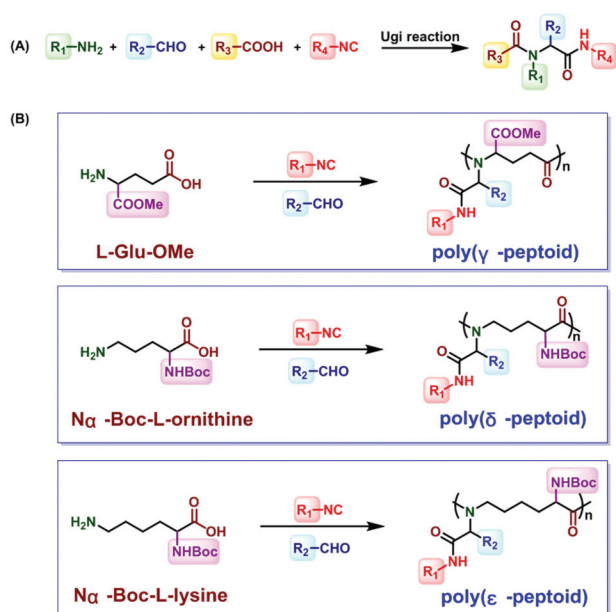
Fig. 3 (A) General formula of the Ugi reaction. (B) Synthesis of poly(γ-, δ- and ε-peptoid)s through the Ugi reaction. 45
