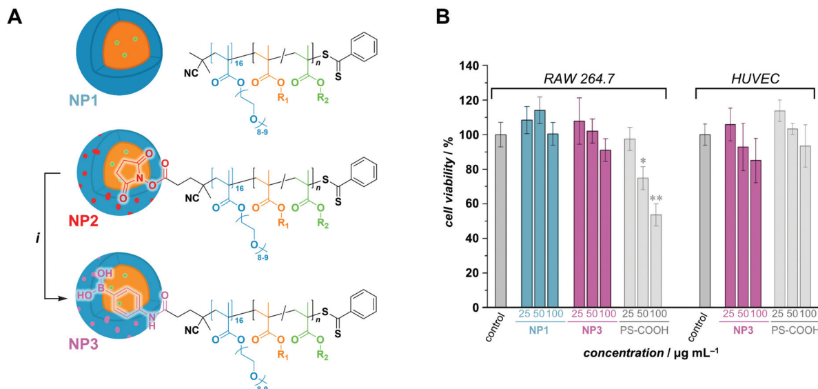
Fig. 4 (A) Modification of NHS ester-functionalized PEOGMA 500 NHS- b -PPBMA nanoparticles. R 1 = 4-phenylboronate pinacol ester; R 2 = fluor- escein. i : 3-aminobenzenboronic acid, triethylamine, ambient temperature. (B) Cell viability of boron-containing PISA-made nanoparticles NP1 and NP3 in RAW 264.7 cells and HUVECs. Data are representative of 2 independent experiments, each performed in triplicates and shown as means ± SEM. *Significantly different from control group (* p < 0.05, ** p < 0.01).
