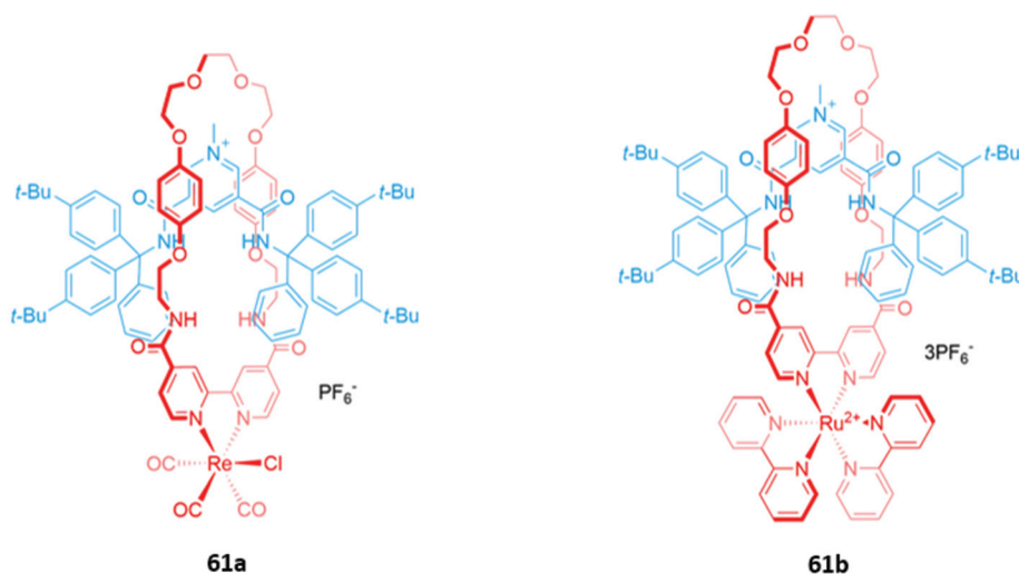
Fig. 35 [2]Rotaxanes with a ruthenium(ii) ( 61a ) or rhenium(i) ( 61b ) complex integrated into the macrocycle which preferentially bind chloride ( K_a > 10^4 \text{ M}^{-1} for 61a in 9 : 1 acetone/ \text{D}_2\text{O} and K_a = 1500 \text{ M}^{-1} for 61b in 7 : 3 acetone/ \text{D}_2\text{O} ).
