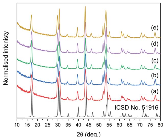
Fig. 1 XRD patterns of synthesised core@shell NPs: (a) NaYF 4 :2% Tm 3+ @NaYF 4 , (b) NaYF 4 :2% Tm 3+ , 5% Er 3+ @NaYF 4 , (c) NaYF 4 :2% Tm 3+ @NaYF 4 :5% Er 3+ , (d) NaYF 4 :18% Yb 3+ , 2% Tm 3+ @NaYF 4 , and (e) NaYF 4 :18% Yb 3+ , 2% Tm 3+ @NaYF 4 :5% Er 3+ . The ICSD reference represents the XRD pattern of β-NaYF 4 with a hexagonal structure.
