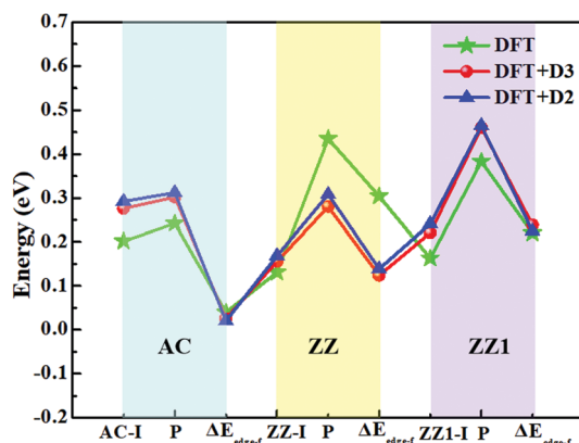
Fig. 3 The edge formation energies (units of \text{eV } \text{\AA}^{-1} ) of the reconstructed edges, AC-I, ZZ-I and ZZI-I, as well as those of pristine AC, ZZ and ZZI edges (expressed by P) calculated by three different methods: DFT, DFT-D3 and DFT-D2. The edge formation energy differences ( \Delta E_{\text{edge-f}} ) between the pristine and reconstructed edges are also presented. The light green, yellow and purple regions indicate AC, ZZ and ZZI edges, respectively.
