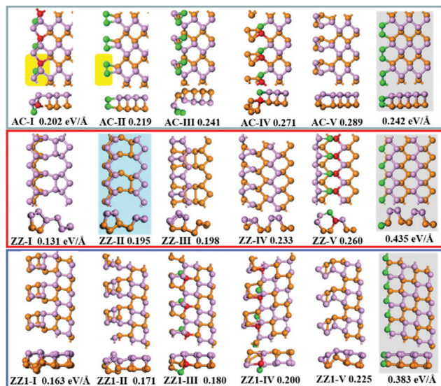
Fig. 2 The highly stable structures of AC, ZZ and ZZI edges together with their edge formation energies (units of \text{eV } \text{\AA}^{-1} ) shown below each configuration. The pristine edge structures without considering edge reconstruction are shown with a gray background. The structure ZZ-II with a light blue background has been reported in the literature. 34 The orange, pink, red and green spheres represent the lower level phosphorus atoms, the upper level phosphorus atoms, and the phosphorus atoms which have four \text{sp}^3 bonds and two \text{sp}^3 bonds, respectively.
