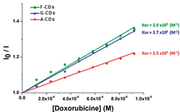
Fig. 32 Stern-Volmer plots of the relative emission intensities ( \lambda_{ex} = 340 nm, \lambda_{em} = 441 nm) of CDs (0.25 mg mL -1 ) as a function of the DOX concentration. Figure reproduced from ref. 155 with permission from American Chemical Society, copyright 2018.
