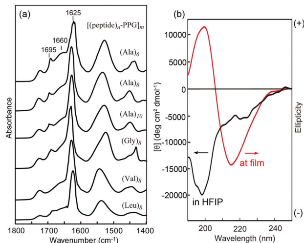
Fig. 2 (a) Transmission FTIR spectra of various [(\text{peptide})_n\text{-PPG}]_m microfilms. (b) CD spectra of [(\text{Ala})_8\text{-PPG}]_m in HFIP ( 2 \text{ mg mL}^{-1} ) and at the film state on a quartz plate.
