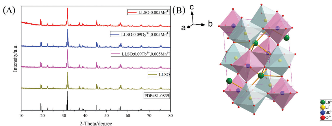
Fig. 1 (A) XRD patterns of \text{LLSO:0.005Mn}^{4+} , \text{LLSO:0.09Tb}^{3+},\text{0.005Mn}^{4+} , \text{LLSO:0.09Dy}^{3+},\text{0.005Mn}^{4+} and LLSO host. (B) Crystal structure schematic diagram of \text{La}_2\text{LiSbO}_6 .
