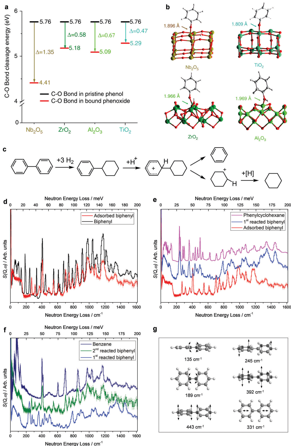
Fig. 3 Conversion of lignin to aromatics. (a) Calculated energies for dissociation of the C–O bonds of phenol upon adsorption over Nb 2 O 5 , ZrO 2 , Al 2 O 3 and TiO 2 . (b) Views of the corresponding DFT-optimised structural models for phenoxide bound on the Nb 2 O 5 (001), ZrO 2 (010), Al 2 O 3 (110) and TiO 2 (101) surfaces. Adapted from ref. 34 published by Springer Nature, licensed under a Creative Commons Attribution 4.0 International License ( https://creativecommons.org/licenses/by/4.0/legalcode ). (c) Possible reaction mechanism in the conversion of biphenyl over the Ru/NbOPO 4 catalyst. Inelastic neutron scattering (INS) spectra for Ru/NbOPO 4 in the adsorption and catalytic conversion of biphenyl. All spectra shown here are difference spectra. (d) Comparison of INS spectra for solid and adsorbed biphenyl on Ru/NbOPO 4 . INS spectra for Ru/NbOPO 4 during the first (e) and second (f) catalytic conversion of biphenyl. (g) Views of selected C–C vibration modes of biphenyl. Reproduced with permission from ref. 35, Copyright© 2019 Elsevier.
