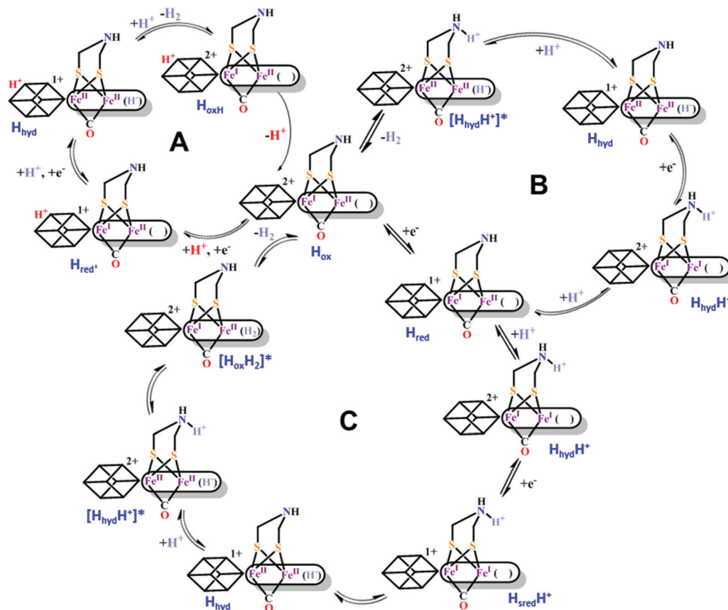
Scheme 22 Proposed catalytic cycles for reversible H + reduction by [FeFe]-hydrogenases. 387–390
