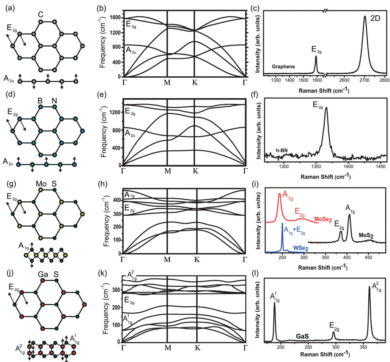
Fig. 1 (a) Top and side (bottom picture) views of the crystal structure of monolayer graphene. (b) Phonon dispersion of graphene showing the high symmetry points and the main phonon modes at the \Gamma point. Phonon dispersion taken from ref. 43. (c) Raman spectrum of graphene with the main Raman peaks. (d and e) The same as in (a and b) but for monolayer h-BN. Phonon dispersion taken from ref. 44. (f) Raman spectrum of few-layer h-BN. (g and h) The same as in (a and b) but for monolayer MoS 2 . Phonon dispersion taken from ref. 45. (i) Raman spectra of monolayer MoS 2 , WSe 2 and MoSe 2 . (j and k) The same as in (a and b) but for GaS. Phonon dispersion taken from ref. 46. (l) Raman spectrum of few-layer GaS. Reproduced with permission from ref. 43–46.
