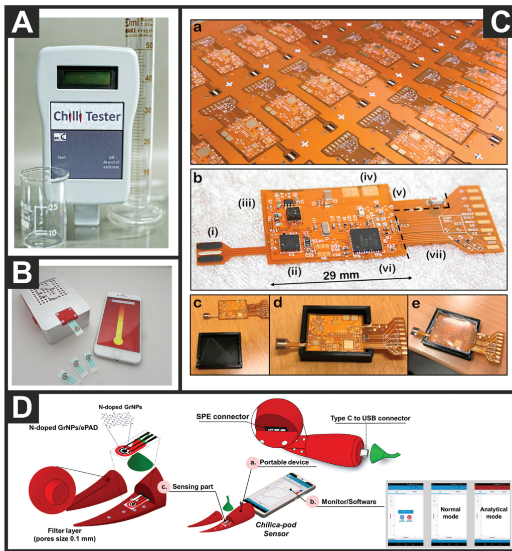
Fig. 4 (A) First in-the-field prototype for measuring the pungency of chiles and chilli products produced by Oxford University. 28 (B) The commercial ChilliPot – the world's first Scoville Meter. 30 (C) Photograph of the electrochemical sensor platform (a) on a 25 × 25 mm panel before component assembly and (b) the single sensor platform after assembly. The Roman numerals indicate (i) the screen-printed electrodes, (ii) the chip potentiostat, (iii) the battery management circuitry, (iv) the terminals for the flexible battery (dimensions 29 × 25 × 0.6 mm) situated on the backside, (v) the antenna circuitry for Bluetooth® Low Energy, (vi) microcontroller with an integrated analog-to-digital converter, and (vii) debug circuitry which can be cut off before deployment. (C–e) Photographs of the encapsulation of the electronic components in a 3D-printed mold. 78 Reproduced with permission from ref. 78. Copyright Elsevier 2019. (D) Components of the Chilica-Pod portable electrochemical capsaicin sensor: (a) body of the portable electrochemical device, (b) monitor/software, and (c) sensor. 54 Reproduced with permission from ref. 54. Copyright American Chemical Society 2020.
