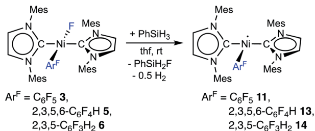
Scheme 7 Synthesis of the metal radicals [Ni I (Mes 2 Im) 2 (C 6 F 5 )] ( 11 ), [Ni I (Mes 2 Im) 2 (2,3,5,6-C 6 F 4 H)] ( 13 ) and [Ni I (Mes 2 Im) 2 (2,3,5-C 6 F 3 H 2 )] ( 14 ).
