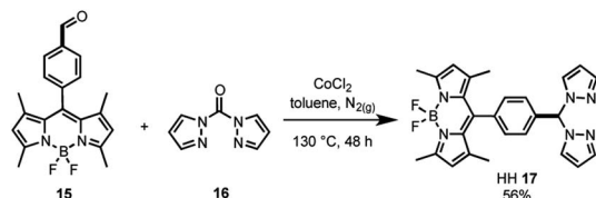
Scheme 2 Synthesis of the bifunctional catalyst framework HH 17.
