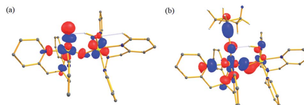
Fig. 9 Computed orbital diagram corresponding to the (a) LUMO of the ^2\mathbf{1}_{ns-hs} and (b) HOMO of the \mathbf{I-}^2\mathbf{TS}_{Hns-hs} .
