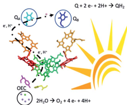
Scheme 1 Map of the main cofactors of water photo-oxidation and reduction of quinones Q_A and Q_B under sunlight irradiation.
