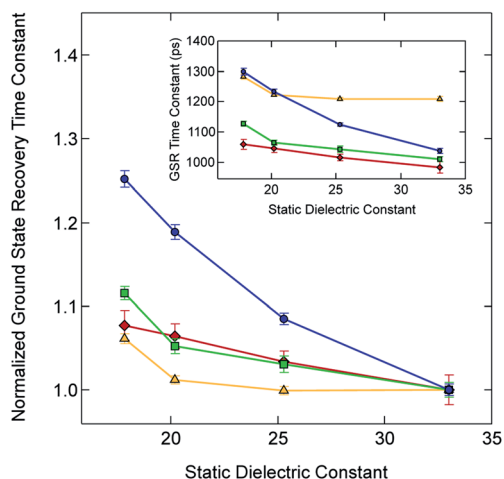
Fig. 6 Time constants for ground state recovery (i.e., ^5T_2 \rightarrow {}^1A_1 conversion) for [\text{Fe}(\text{bpy})_3]^{2+} (red diamonds), [\text{Fe}(\text{dmb})_3]^{2+} (yellow triangles), [\text{Fe}(5,5'\text{-dmb})_3]^{2+} (green squares) and [\text{Fe}(\text{dtbbpy})_3]^{2+} (blue circles) in alcohol-based solutions, normalized to each complex's ground state recovery lifetime in methanol. The solid line between each data point is not a fit but is merely present to guide the eye. The inset shows the raw data listed in Table 3. See text for further details.
