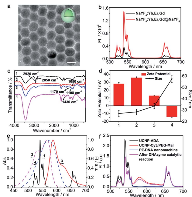
Fig. 1 (a) TEM image of \text{NaYF}_4:\text{Yb,Er,Gd}@/\text{NaYF}_4 UCNP (scale bar: 20 nm). (b) Upconversion luminescence spectra of \text{NaYF}_4:\text{Yb,Er,Gd} and \text{NaYF}_4:\text{Yb,Er,Gd}@/\text{NaYF}_4 under 980 nm excitation. (c) FTIR spectra of (1) UCNPs-OA, (2) UCNPs-ADA, (3) UCNPs-Cy3/PEG-Mal, and (4) the PZ-DNA nanomachine. (d) Zeta potential and DLS analysis of (1) bare UCNP, (2) UCNPs-ADA, (3) UCNPs-Cy3/PEG-Mal, and (4) the PZ-DNA nanomachine. The error bars indicate means \pm S.D. ( n = 3 ). (e) Normalized fluorescence emission spectra (solid lines) of (1) UCNP under 980 nm excitation and (3) Cy3 under 540 nm excitation, along with normalized absorption spectra (dashed lines) of (2) Cy3 and (4) BHQ2. (f) Normalized upconversion luminescence spectra of UCNPs-ADA, UCNPs-Cy3/PEG-Mal, and the PZ-DNA nanomachine before and after the DNAzyme catalytic reaction.
