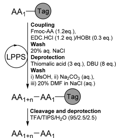
Fig. 8 Ajiphase® soluble anchors for liquid-phase peptide synthesis (LPPS) developed by Takahashi et al. and commercialised by Ajinomoto Bio-Pharma Services 105–107
