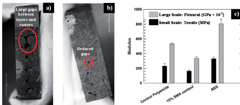
Fig. 14 SEM analysis of the fracture surfaces for BAAM samples (a) PA, (b) PA/ABS compatibilized and (c) a comparison of moduli for small scale versus large scale printing. 7 Reprinted with permission from Elsevier: Additive Manufacturing , Copyright 2019, License: 4694241403414.
