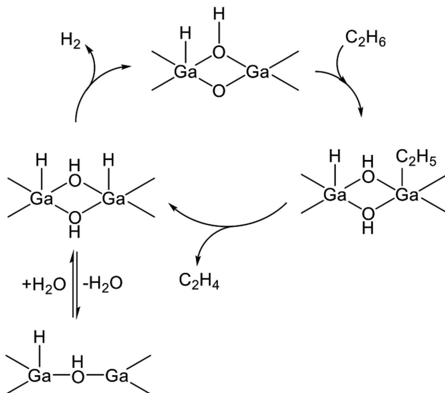
Scheme 4 Reaction mechanism of EDH in the presence of steam on a Ga oxide cluster.
