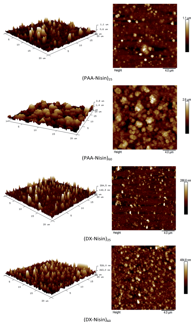
Fig. 6 Atomic force microscope (AFM) height images ( 20 \mu\text{m} by 20 \mu\text{m} ) of the 25 and 60 bilayer films of PAA-nisin and DX-nisin.
