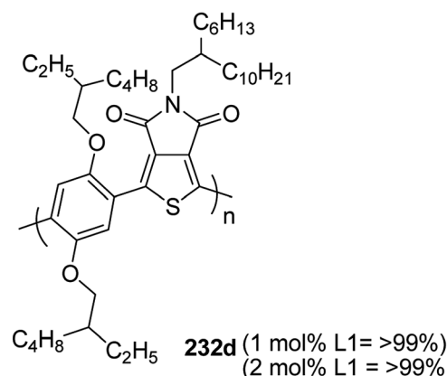
Scheme 68 Polycondensation of dibromoarenes and thieno[3,4-c]pyrrole-4,6-dione via direct arylation polymerization to synthesize 232a–d .
