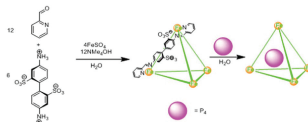
Fig. 25 Synthesis of cage \text{II}^{\text{Fe}} and trapping of white phosphorus ( \text{P}_4 ) within tetrahedral cage \text{II}^{\text{Fe}} . Reproduced with permission from ref. 42. Copyright 2009, American Association for the Advancement of Science.
