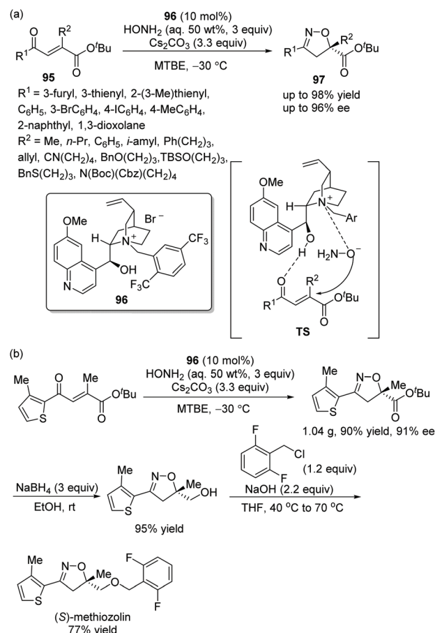
Scheme 34 Oxa-Michael cascade reaction for the synthesis of chiral isoxazolines and the derivatization of the chiral product.
