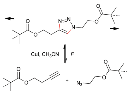
Scheme 19 Supposed force-induced cycloelimeration of the triazole mechanophore yielding azide and alkyne moieties. 98,99
