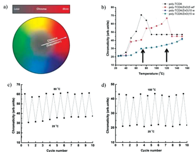
Fig. 16 (a) Schematic showing chromaticity distribution from dull to vivid. (b) Chromaticity versus temperature plots for TCDA and TCDA/ZnO composites. (c) Chromaticity of TCDA/ZnO (5 wt%) as a function of thermal cycle. (d) Chromaticity of TCDA/ZnO (15 wt%) as a function of thermal cycle. Reproduced from ref. 58 with permission from the American Chemical Society, copyright [2013].
