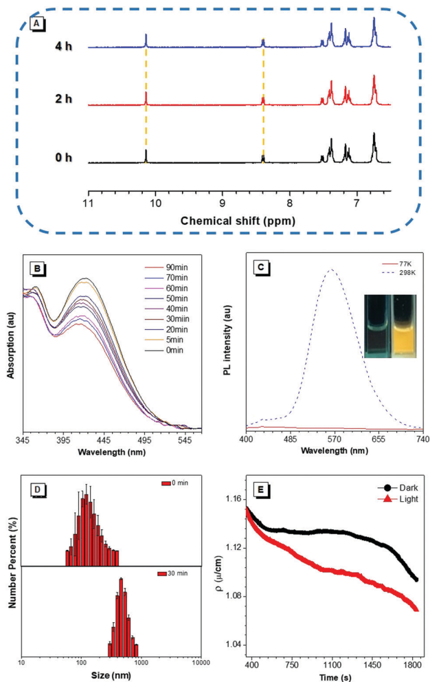
Fig. 2 (A) Change of 1 H NMR spectra of TIOdB in the DMSO- d 6 solution ( 2 \times 10^{-3} M) before and after 365 nm, 2.48 mW cm -2 UV light from a hand-held UV lamp for 0, 2 h, and 4 h. (B) UV spectra of TIOdB (10 μM) in the DMSO solution irradiated with 365 nm, 2.48 mW cm -2 UV light from a hand-held UV lamp for different times. (C) PL spectra of TIOdB (10 μM) in the DMSO solution after irradiation with 365 nm, 2.48 mW cm -2 UV light from a hand-held UV lamp for 30 min at 77 and 298 K respectively. (D) DLS results before and after irradiation for 10 min in aqueous solutions. (E) The conductivity of TIOdB in aqueous solutions with different light illumination time and in dark condition. Concentration: 10 μM.
