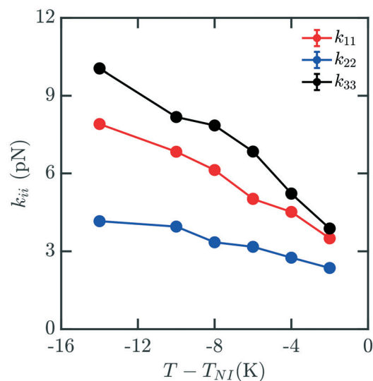
Fig. 5 Bulk elastic constants for a mixture with of 5CB and 8CB with mole fractions x_{5CB} = x_{8CB} = 0.5 .
