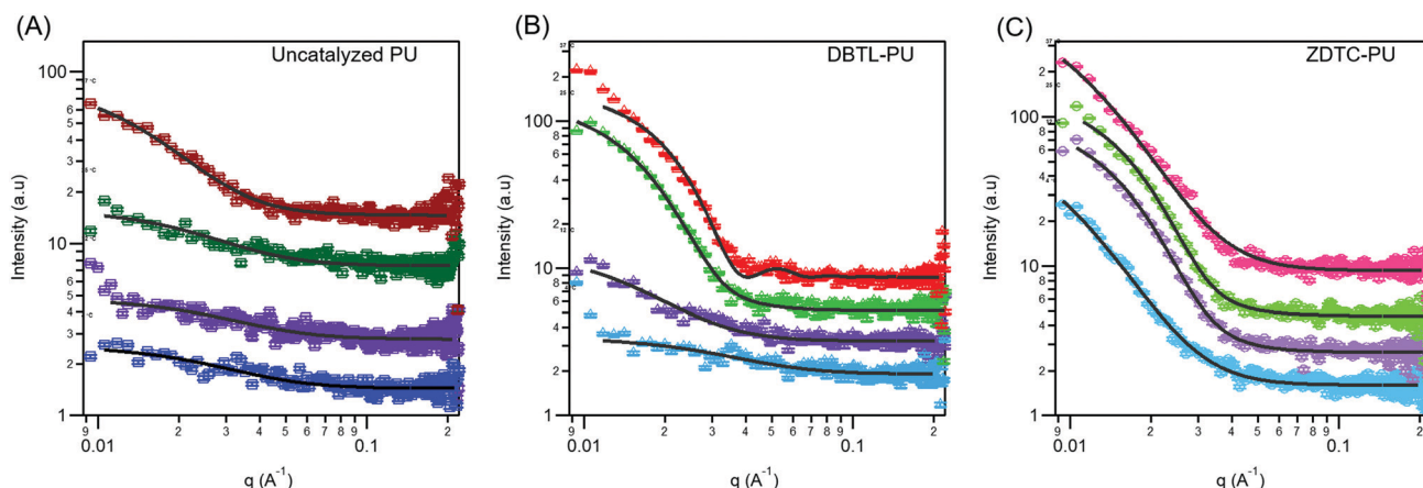
Fig. 6 Small-angle X-ray scattering patterns of 2 wt/v% aqueous solutions of (A) uncatalysed PUs ( \square ); (B) DBTL-catalysed PUs ( \Delta ) and (C) ZDTC-catalysed PUs ( \circ ) at 4, 12, 25 and 37 °C. The solid black lines are model fits to the data. Curves are offset for clarity.
