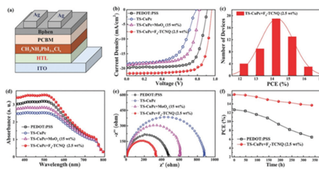
Fig. 18 (a) Schematic diagram of the device structure in inverted PSCs incorporating different HTMs; (b) J - V curves of the PSCs using PEDOT:PSS, TS-CuPc, TS-CuPc:MoO 3 (15 wt%) and TS-CuPc: F_4 -TCNQ (2.5 wt%) as the HTMs measured under simulated AM 1.5 sunlight of 100 \text{mW cm}^{-2} ; (c) histogram of PCEs measured from 50 TS-CuPc: F_4 -TCNQ (2.5 wt%)-based inverted PSCs; (d) UV-vis absorption spectra of \text{CH}_3\text{NH}_3\text{PbI}_{3-x}\text{Cl}_x perovskite films deposited on different HTMs; (e) Nyquist plots of \text{CH}_3\text{NH}_3\text{PbI}_{3-x}\text{Cl}_x -based PSCs measured in the dark, at an applied voltage of 0.96 V; (f) PCEs as a function of time in the PEDOT:PSS and TS-CuPc: F_4 -TCNQ (2.5 wt%)-based PSCs without encapsulation under identical storage conditions (in atmosphere, at RT). 123
