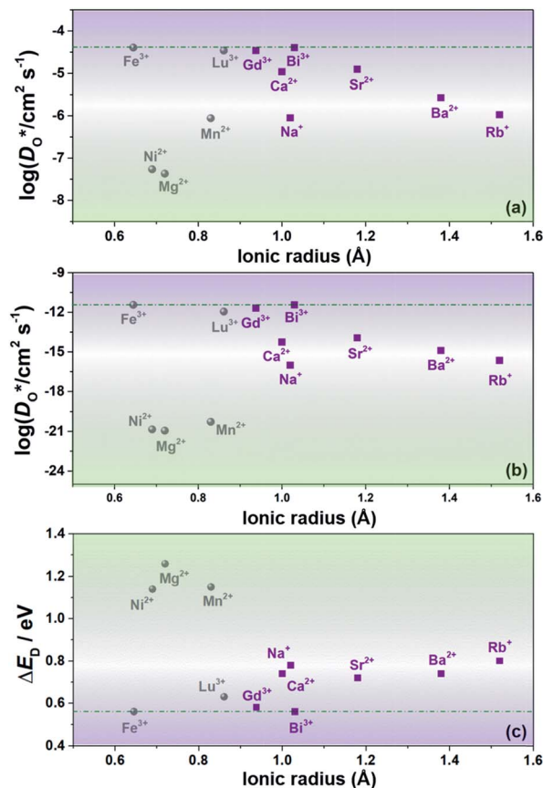
Fig. 4 Oxygen diffusion in substituted, rhombohedral BiFeO 3 : (a) D_o^* extrapolated to T = 1000 K; (b) D_o^* extrapolated to T = 300 K; (c) activation energy of diffusion. The dashed lines correspond to the values for pure BFO (Bi 3+ and Fe 3+ are also plotted for reference). Purple denotes substituents for the A site, whilst silver denotes substituents for the B site.
