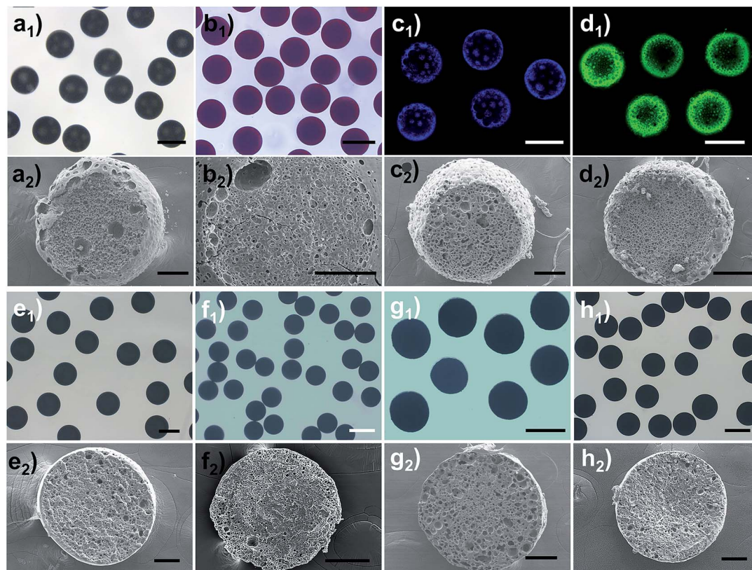
Fig. 8 Great extensibility of our proposed osmotically driven phase separation. Optical and SEM images of the formed pore-structured spheres by using C_{30}\text{vim}[\text{Tf}_2\text{N}]-\text{LiTf}_2\text{N} as a general phase separation carrier platform for realizing the phase separation of various substances: (a 1–2 ) ETPTA, (b 1–2 ) azobenzene-type monomer, (c 1–2 ) AIE-type monomer, (d 1–2 ) bioorthogonal monomer (click reaction with GOX-FITC enzyme), (e 1–2 ) \text{TiO}_2 particles, (f 1–2 ) Au nanoparticles, (g 1–2 ) carbon nanotubes, and (h 1–2 ) graphene. Scale bars are 400 \mu\text{m} (a 1–h1 ) and 100 \mu\text{m} (a 2–h2 ).
