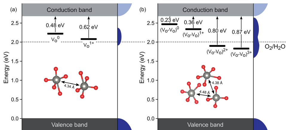
Fig. 3 Defect ionisation levels of oxygen vacancies in different charge states calculated from hybrid density functional theory for (a) an isolated oxygen vacancy V_{O(y)} and (b) a defect complex composed of two oxygen vacancies V_{O(zy)} . Energies are relative to the valence band edge. Densities of states are illustrated schematically at the right side of each panel. The insets show local atomic structures and the distance between the W atoms.
